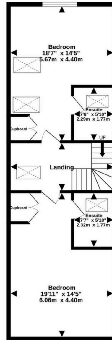
1st Floor 653 sq.ft. (60.7 sq.m.) approx.
